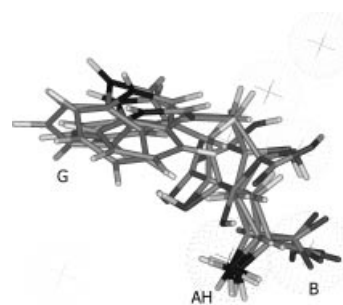
Figure 5. The four stereoisomers of monatin superimposed on the MPA model. Glucophores are indicated by grey-dot spheres; only AH, B and G are labeled for clarity.
