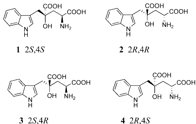
Figure 1. The four stereoisomers of monatin.
