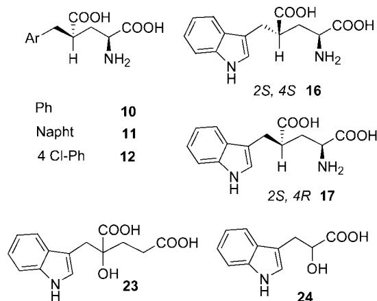
Figure 3. Tasteless monatin analogues.
