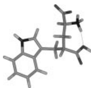
Figure 4. Minimum energy conformation of deoxyderivative 17 .
