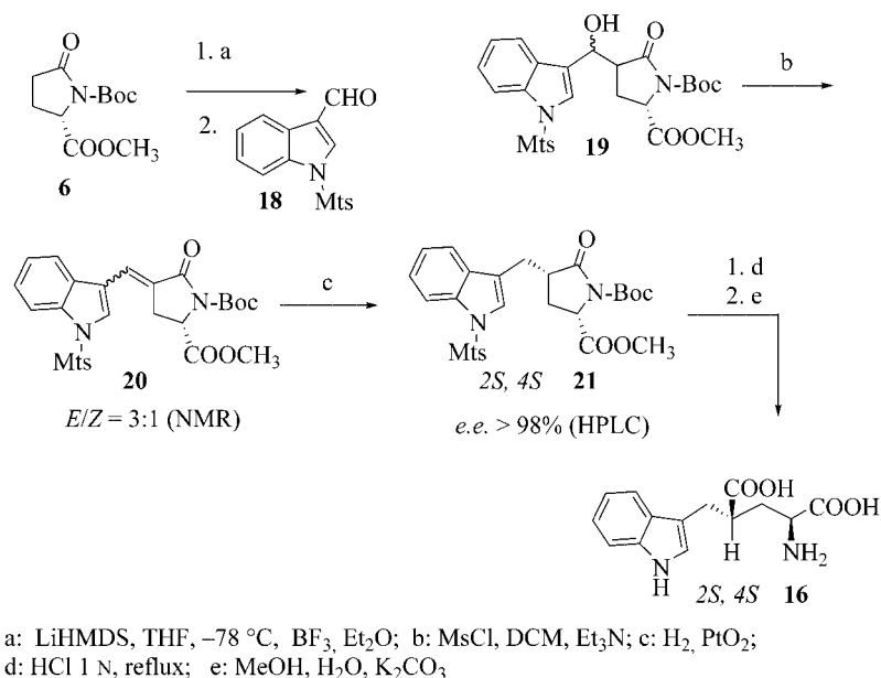
Scheme 3. Synthesis of compound 16 by aldol condensation.
