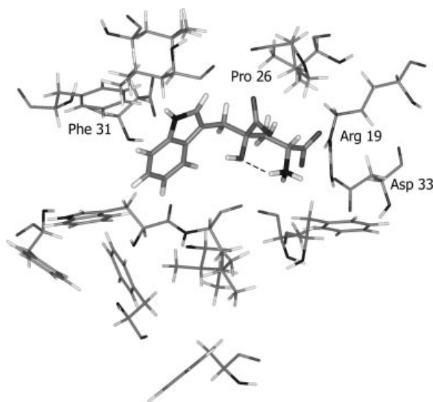
Figure 6. 2 R ,4 R monatin (compound 2 ) in the pseudoreceptor cavity.
