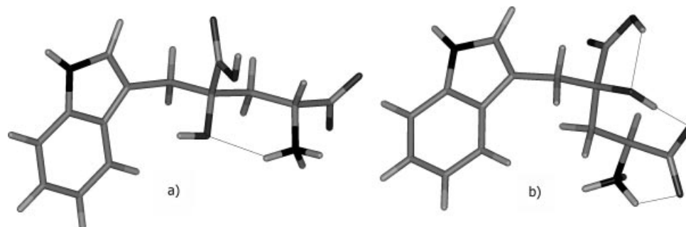
Figure 2. Minimum energy conformations: a) 2 R * ,4 R * monatin; b) 2 R * ,4 S * monatin.
