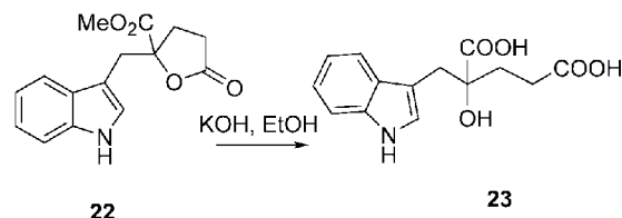
Scheme 4. Synthesis of deamino derivative 23 .
